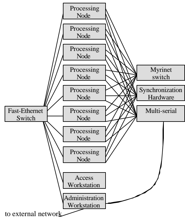
Fig. 3. PAD Cluster Architecture
