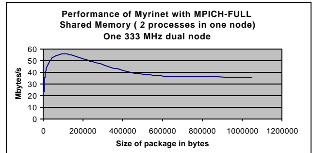
Fig. 6. Intranode communication
