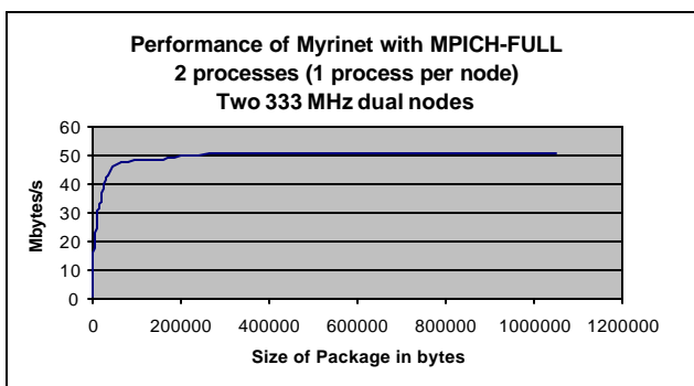
Fig. 5. Internode communication
