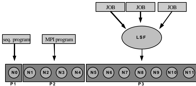
Fig. 10. Example of job scheduling over one partition
