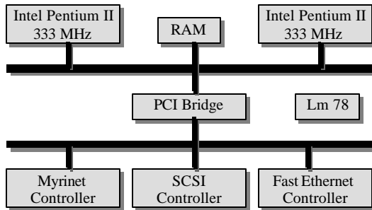
Fig. 4. Node Architecture
